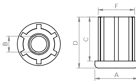
ROUND THREADED TUBE ENDS
